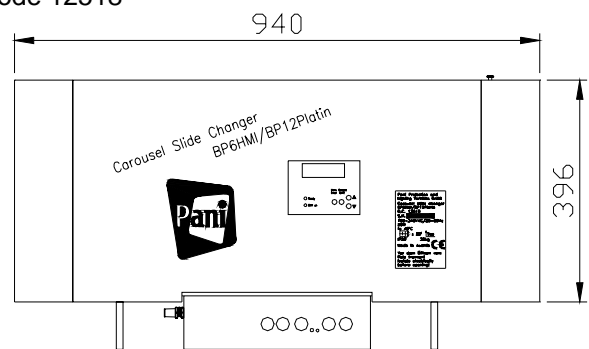
2) position drawing
